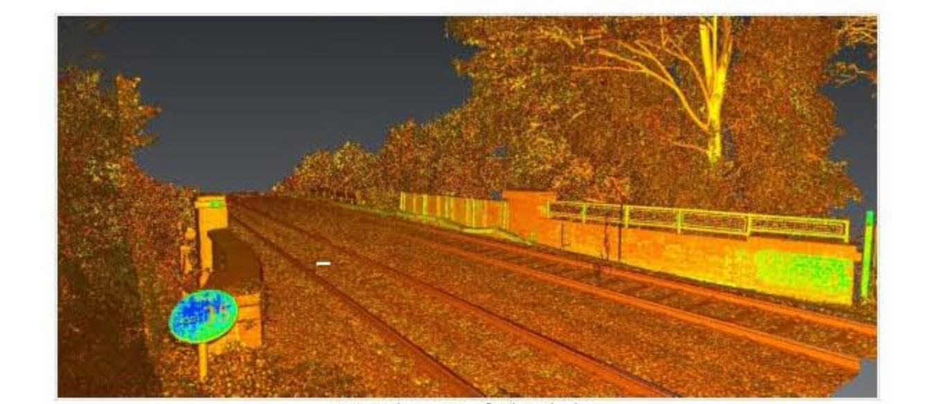
Recent laser scan of railway bridge
